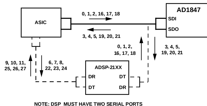
Figure 8. Time Slot Allocation Example
