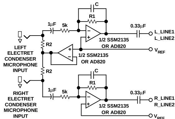
Figure 16. "Phantom-Powered" Microphone Input Circuit
