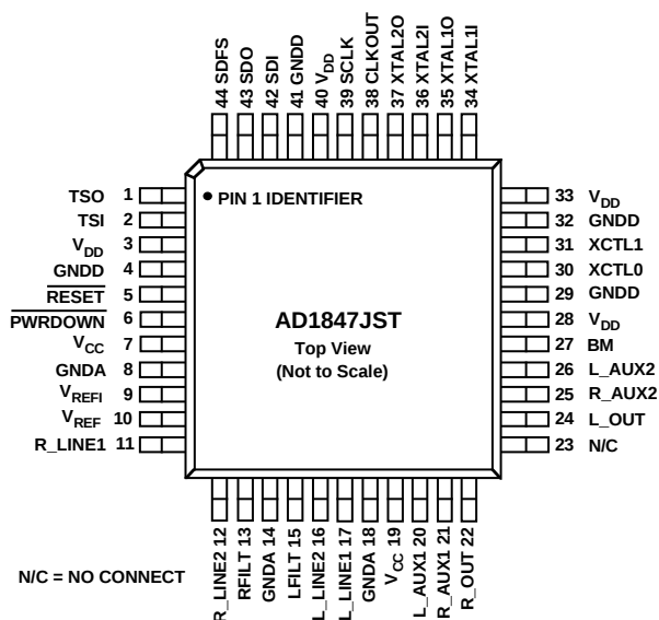
44-Lead TQFP
